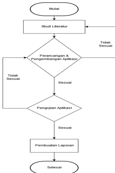
Figure 3.1 Flowchart
